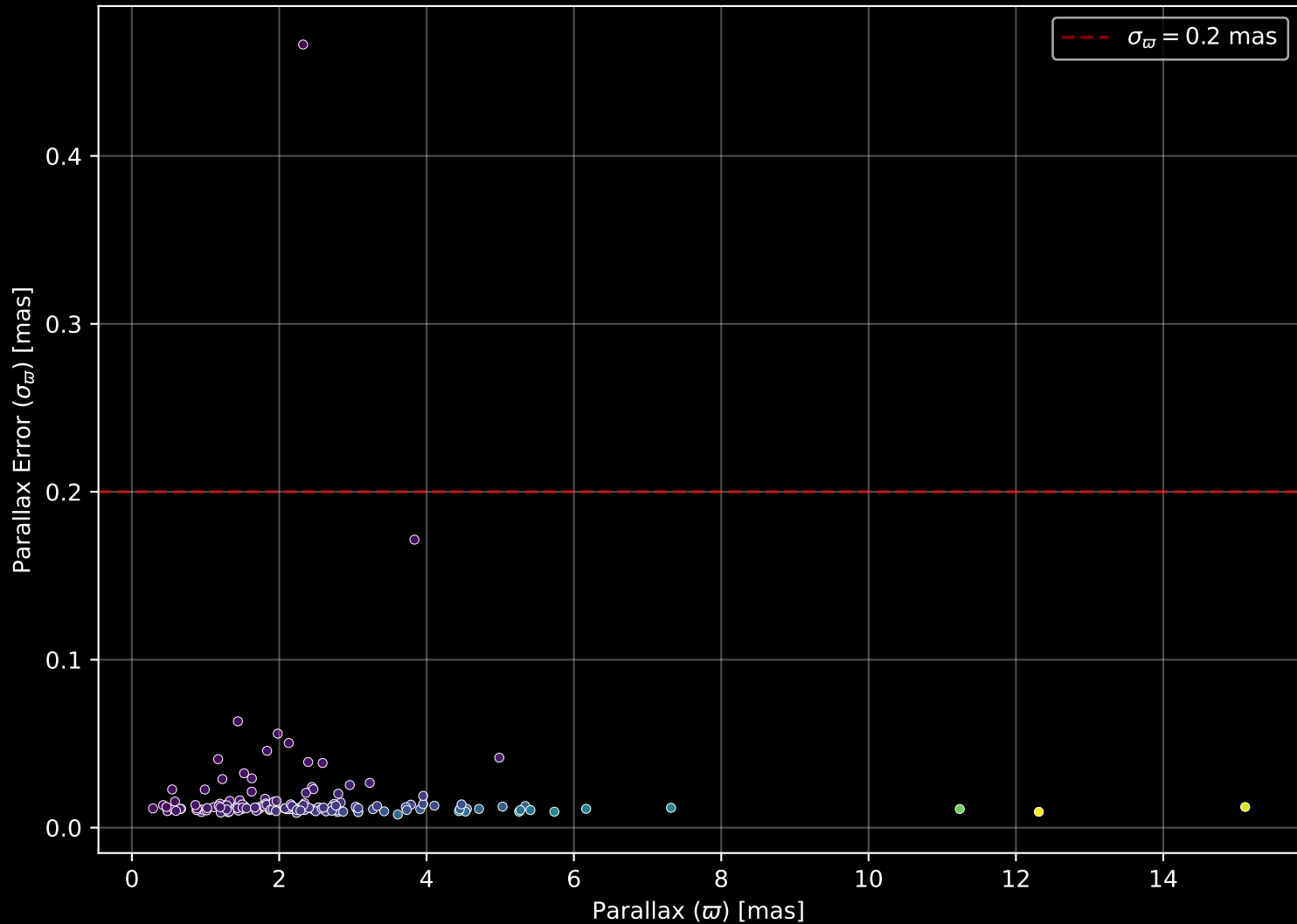
GALAH DR4 Field: [7242] Parallax Quality (n= 144)
