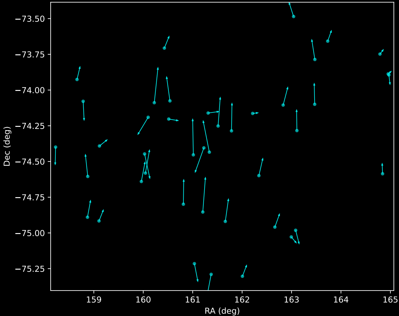
GALAH DR4 Noise Stream Proper Motion Vectors (n=42)
