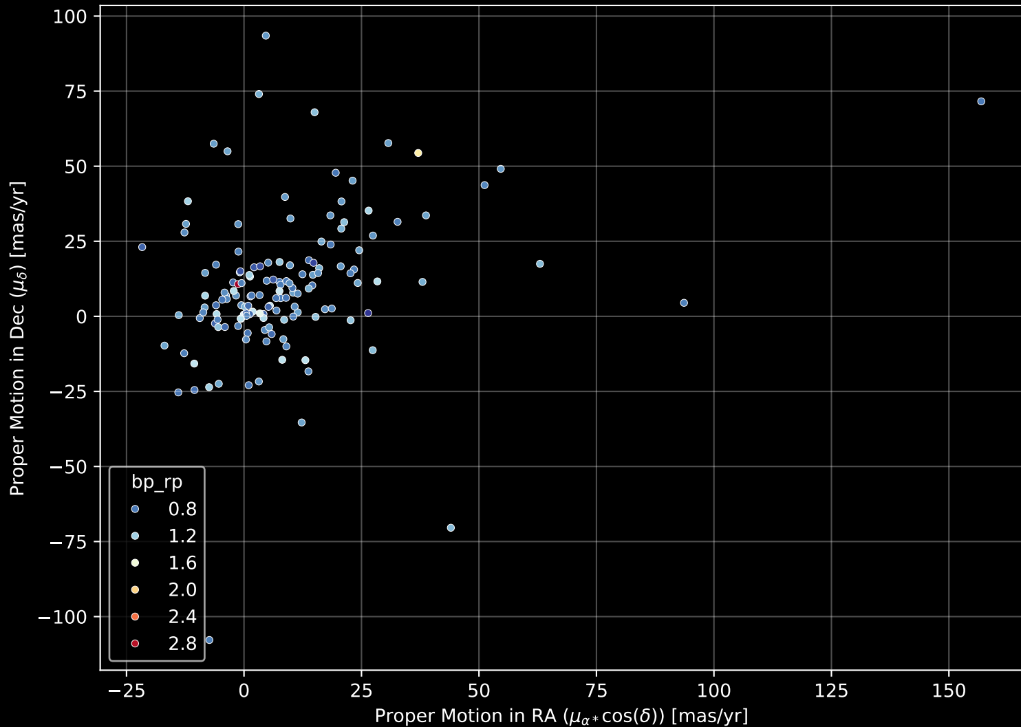
GALAH DR4 Field: [7242] Proper Motion Diagram (n= 144)
