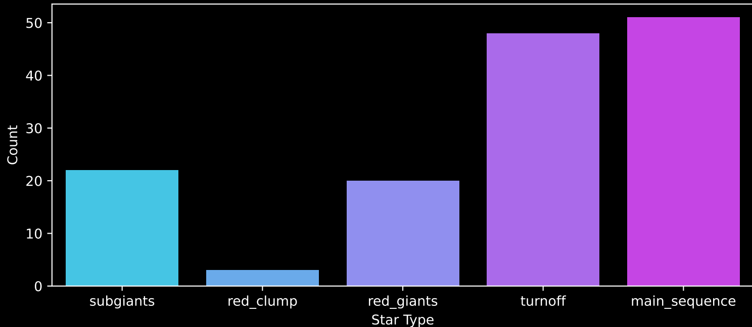
GALAH DR4 Field: [7242] Count plot of Star Type
