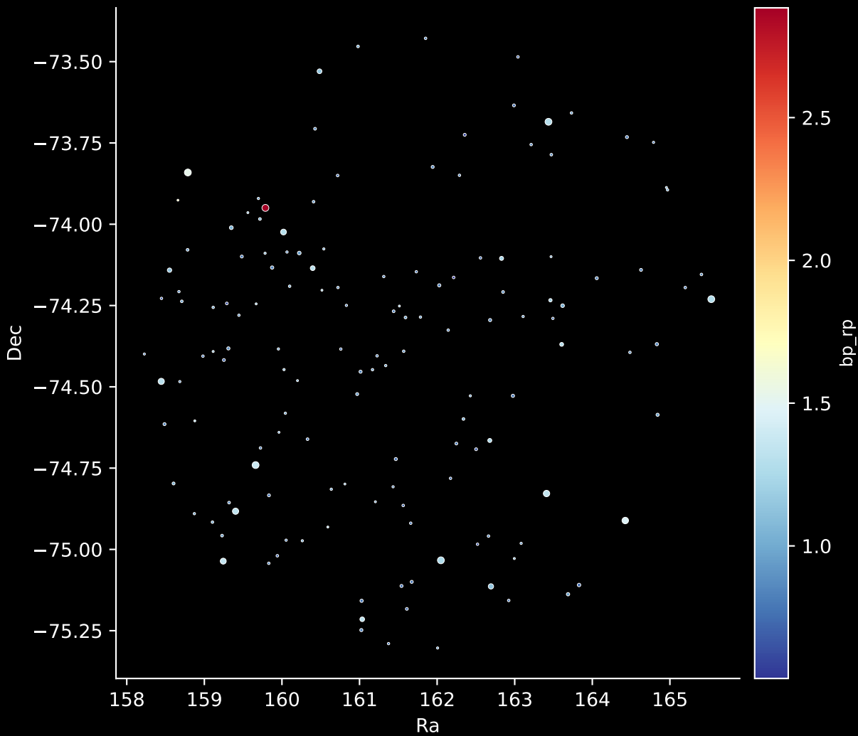
GALAH DR4 Field: [7242] Stars: 144
