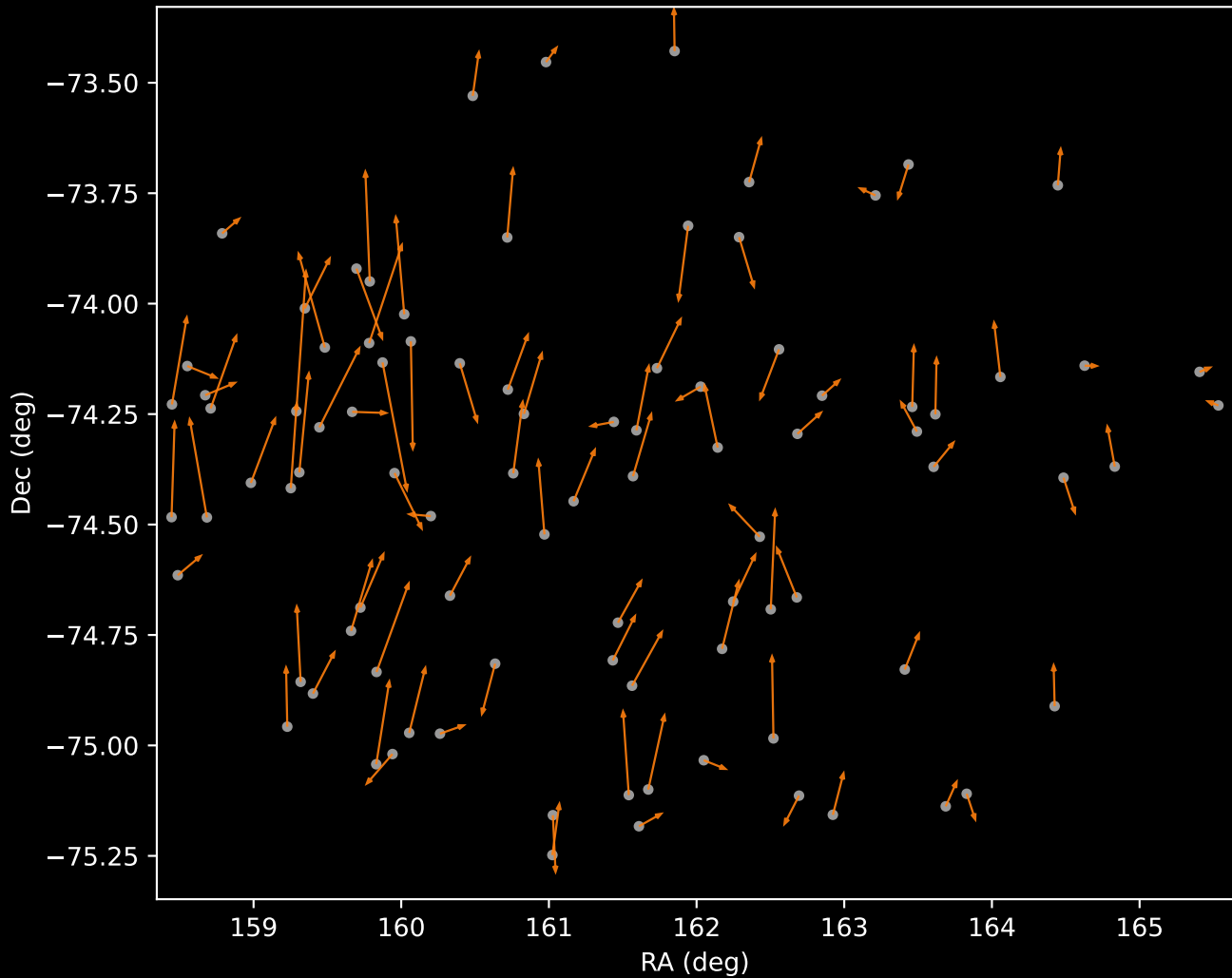
GALAH DR4 Cluster 2 Proper Motion Vectors (n=92)
