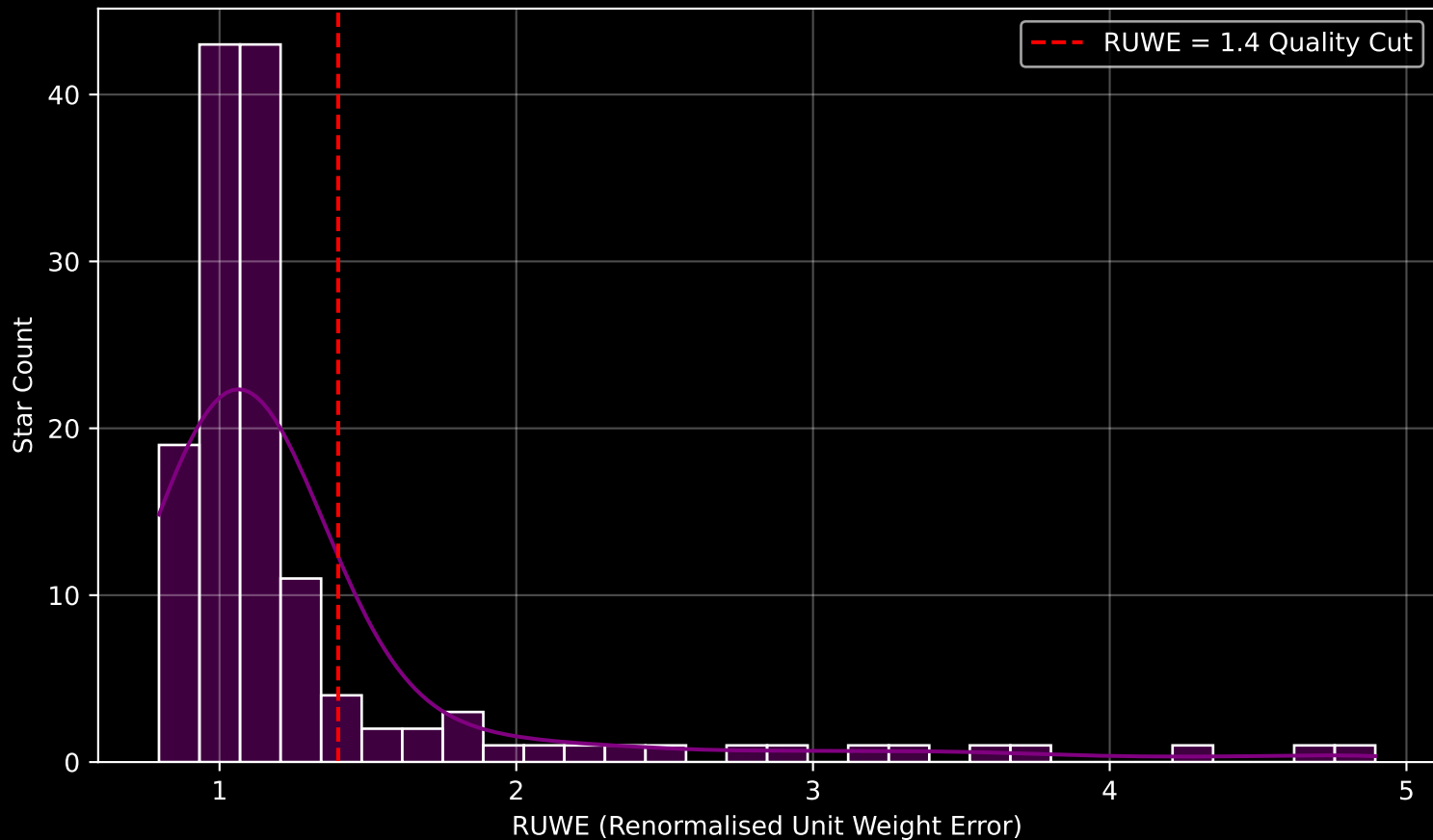
GALAH DR4 Field [7242] RUWE Distribution (n= 141)
