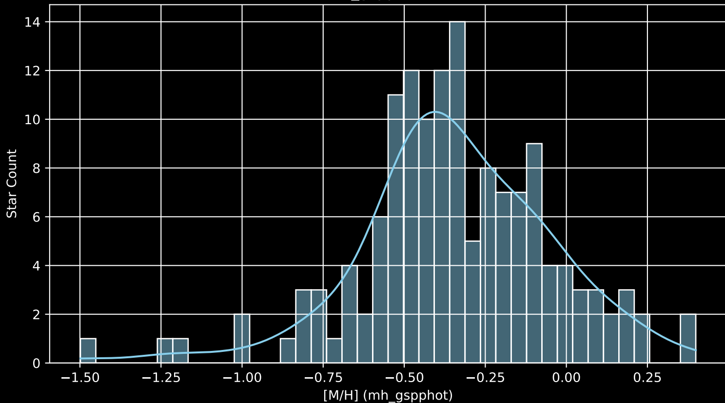
GALAH DR4 Field: [7242] [M/H] (mh_gspphot) (n= 143)
